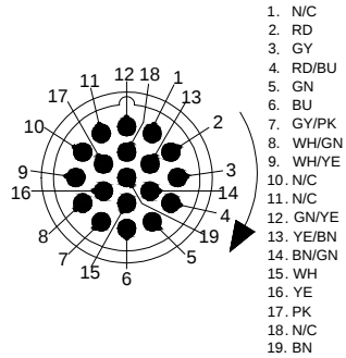
MALE END VIEW
